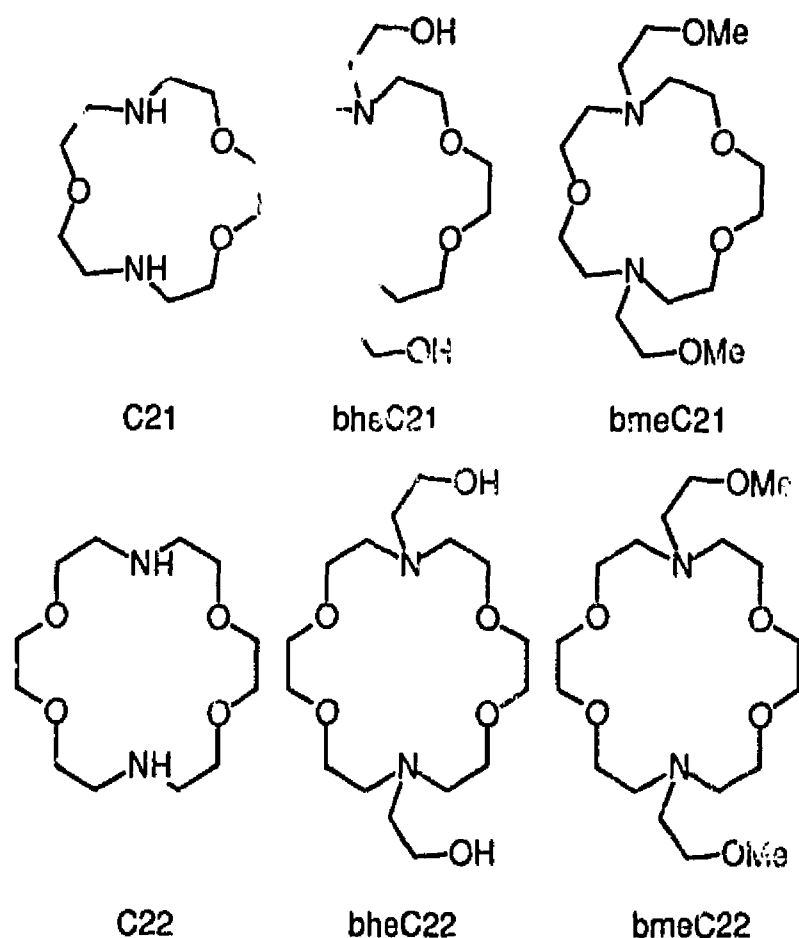
Fig. 2. Schematic representations of some diaza coronands and bibracchial lariat ethers.
