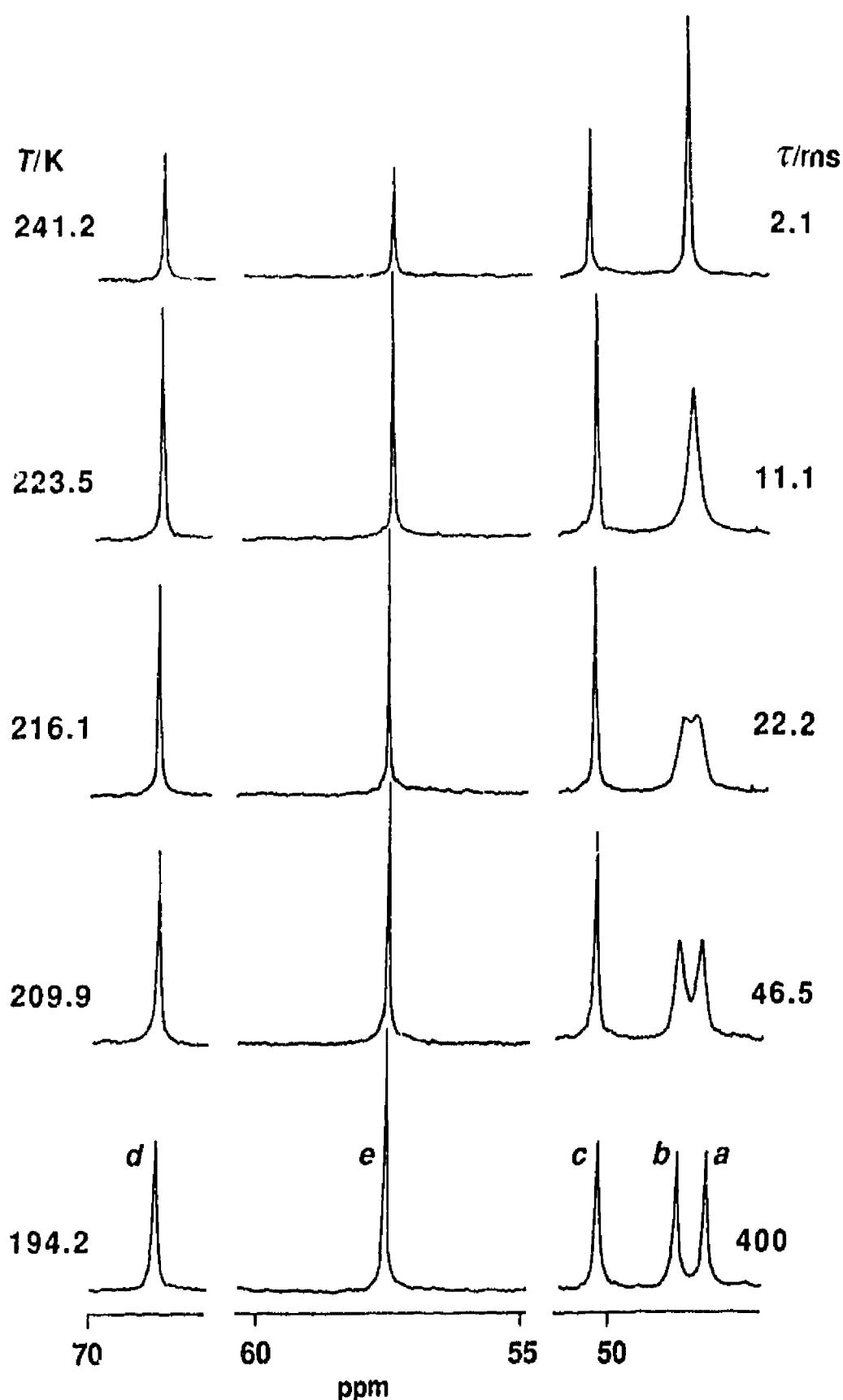
Fig. 8. Exchange modified 75.47 MHz ^{13}\text{C} NMR spectra of 0.10 \text{ mol dm}^{-3} [\text{Li}(\text{tmecl}_2)\text{ClO}_4] in ^{12}\text{C} -enriched [\text{}^2\text{H}_4] methanol. Experimental temperatures and derived site lifetimes, \tau , appear to the left and right of the figure (adapted from Ref. [119]).
