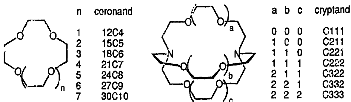
Fig. 1. Schematic representations of coronands and cryptands.
