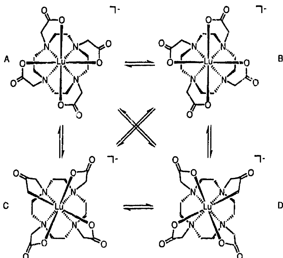
Fig. 9. The enantiomerisation and isomerisation of the major (A and B) and minor (C and D) [\text{Lu}(\text{dota})]^- isomers showing the macrocyclic ring conformations. The capping coordinated water is not shown.
