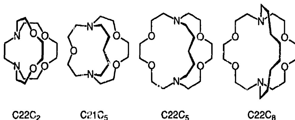
Fig. 3. Schematic representations of some modified cryptands.
