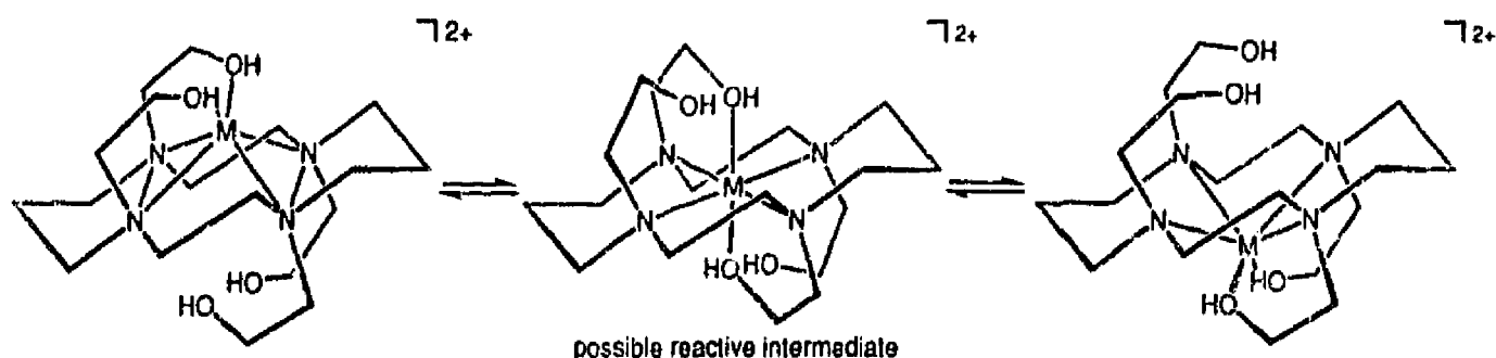
Fig. 10. The transannular exchange mechanism proposed for [Cd(thecl4)] 2+ , and its Hg 2+ and Pb 2+ analogues.
