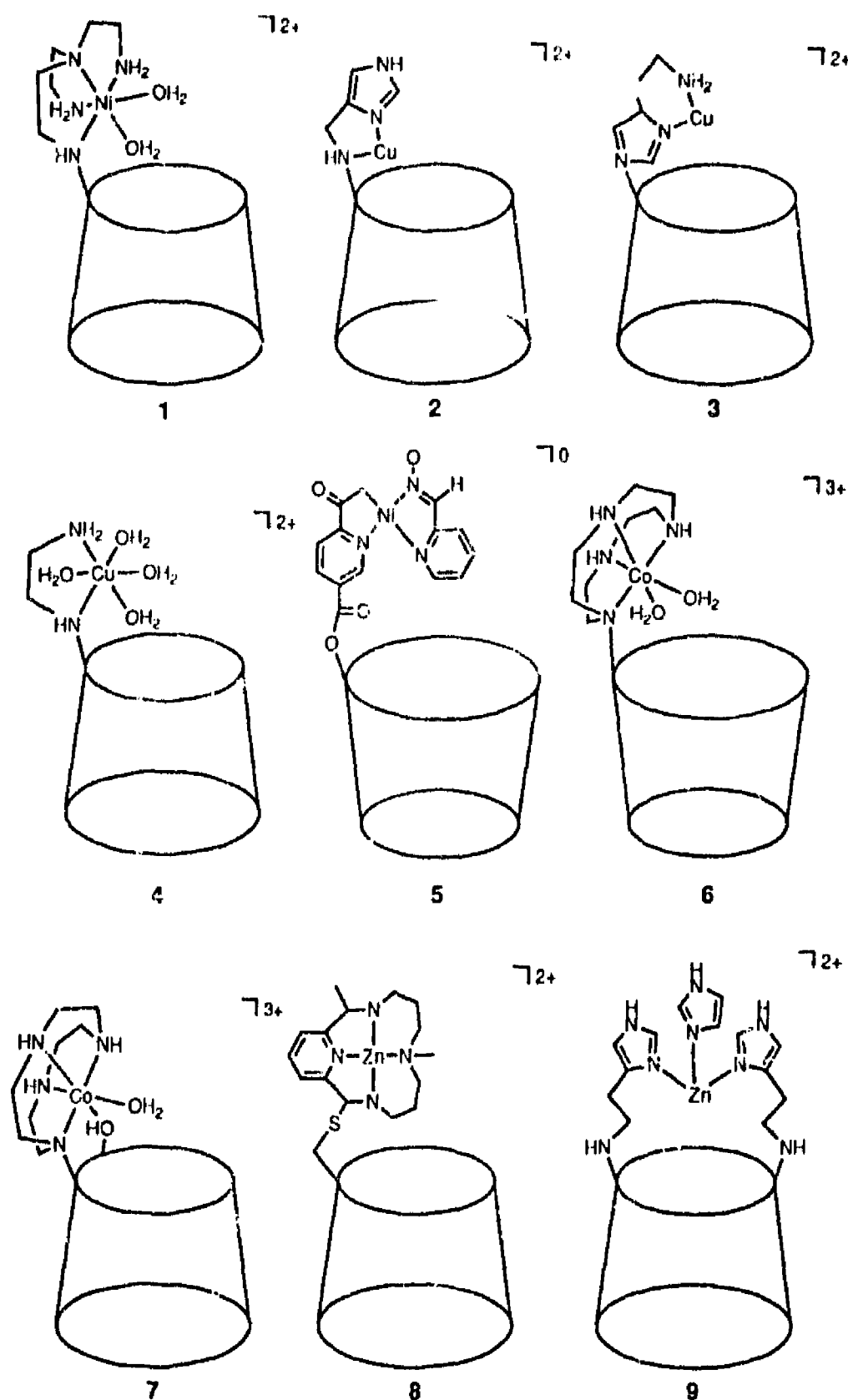
Fig. 14. Schematic representation of some metallocyclodextrins.
