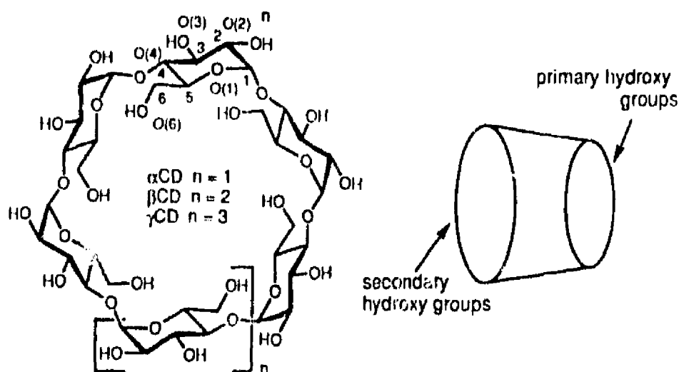
Fig. 12. Schematic representation of \alpha -, \beta - and \gamma -cyclodextrin whose internal annular diameters measured from the C(5) hydrogens are 470, 600 and 750 pm, respectively, and 520, 640 and 830 pm measured from the C(3) hydrogens in Corey Pauling Koltun models. The depths of the annuli measured between the rings delineated by the primary and secondary hydroxyl groups are 790–800 pm [14, 17]. Their representation as a truncated cone is also shown. A substituent drawn at either the narrow or wide end of the cone indicates that it has either replaced a C(6) hydroxyl group, or a C(2) or a C(3) hydroxyl group.
