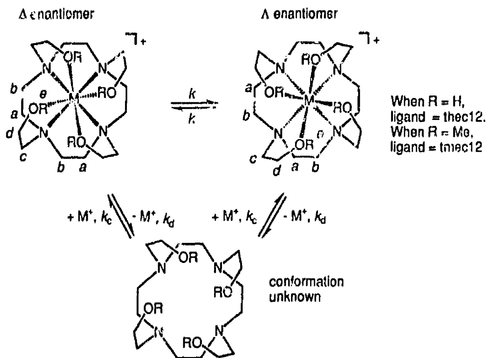
Fig. 6. Enantiomerisation of \Delta and \Lambda[M(\text{thec12})]^+ and \Delta and \Lambda[M(\text{tmec12})]^+ and M^+ exchange in both systems. The \Delta and \Lambda enantiomers are those where the pendant arms assume a clockwise and anticlockwise chirality, respectively, when the structure is viewed from the centre of the four oxygen plane looking towards M^+ and the nitrogen plane beyond.
