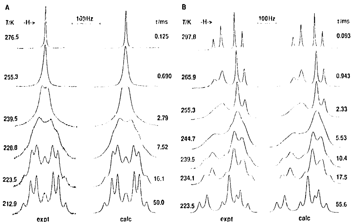
Fig. 11. The exchange modified ^{13}\text{C} 75.47 MHz NMR spectra of the 99% ^{13}\text{C} enriched 2-hydroxyethyl arms of (A) [\text{Cd}(\text{thecl4})]^{2+} and (B) [\text{Pb}(\text{thecl4})]^{2+} in \text{CD}_3\text{OD} . The experimental temperatures and derived mean lifetimes of the 2-hydroxyethyl arms in the mono- and bidentate environments appear to the left and right of each figure, respectively. For [\text{Cd}(\text{thecl4})]^{2+} J(^{13}\text{C}-^{13}\text{C}) = 39.0 and 39.3 Hz for the downfield and upfield quartets, respectively. For [\text{Pb}(\text{thecl4})]^{2+} J(^{13}\text{C}-^{13}\text{C}) = 40.5 and 40.2 Hz for the downfield and upfield quartets, respectively (adapted from Refs. [144] and [145]).
