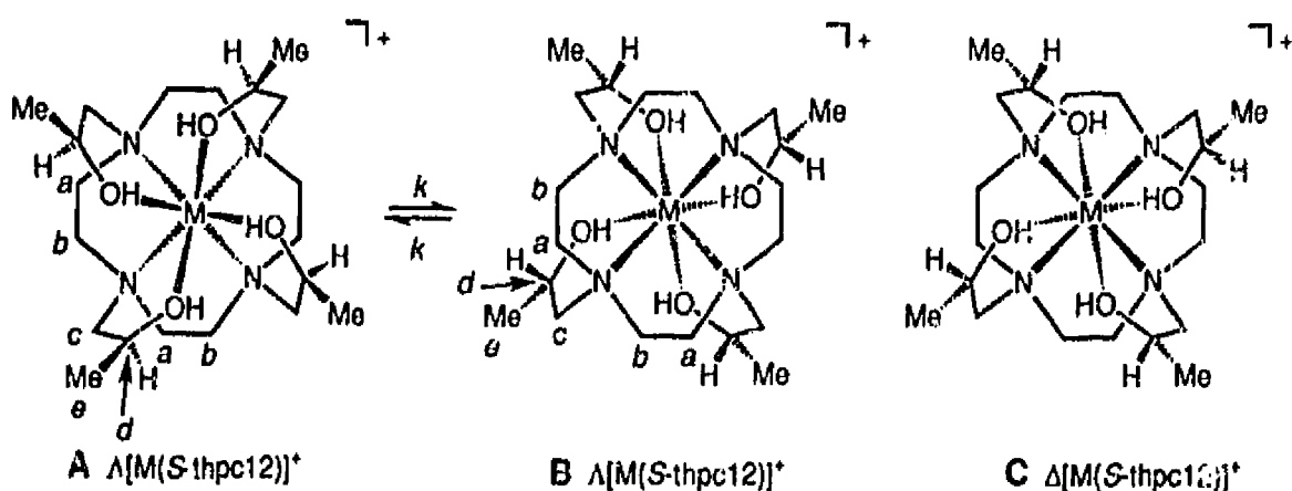
Fig. 7. The exchange process for equivalent forms of the \Lambda[\text{Na}(\text{S-thpc12})]^+ diastereomer, A and B, leading to the exchange of the macrocycle carbons between environments a and b. The undetected \Delta[\text{Na}(\text{S-thpc12})]^+ diastereomer is shown as C. The \Delta and \Lambda diastereomers are those where the pendant arms assume a clockwise and anti-clockwise chirality, respectively, when the structure is viewed down the C_4 axis from the four oxygen plane looking towards \text{Na}^+ and the nitrogen plane beyond. The rotation of the plane delineated by the four oxygens away from eclipsing that delineated by the four nitrogens is exaggerated for illustration purposes.
