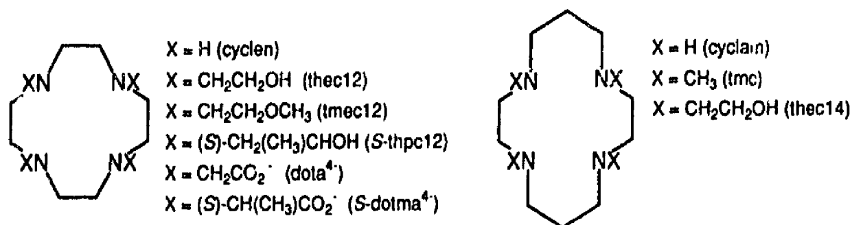
Fig. 5. Schematic representations of some tetraaza-macrocyclic ligands.
