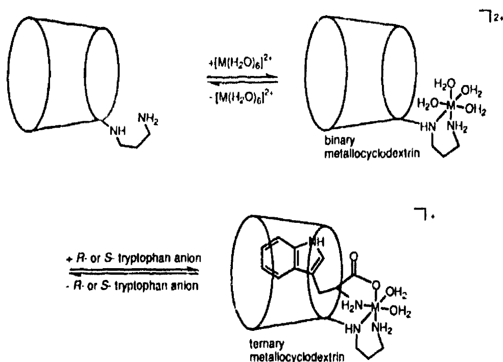
Fig. 13. The formation of binary and ternary metallocyclodextrins by 6^A -(3-aminopropylamino)- 6^A -deoxy- \beta -cyclodextrin.
