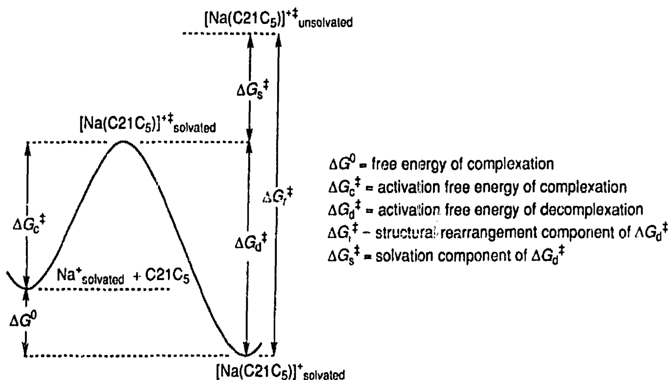
Fig. 4. Free energy profile for [\text{Na}(\text{C21C}_5)]^+ .
